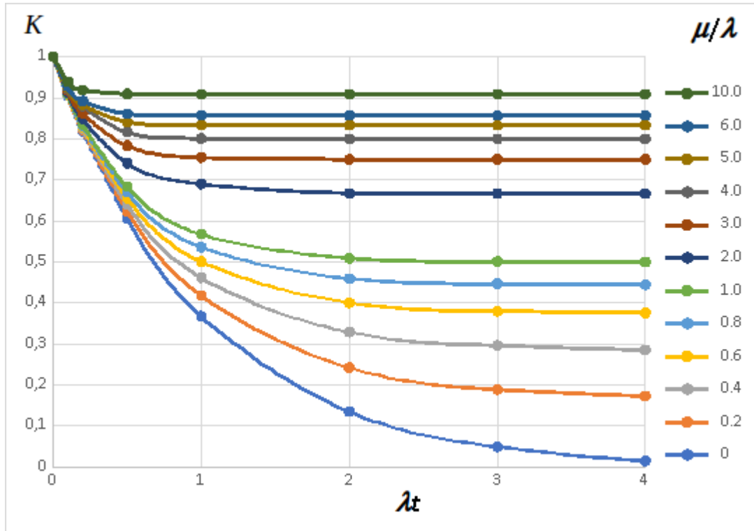
Fig.1. Availability function K(t) vs the product \lambda t of failure rate and time for different restoration-to-failure-rate ratios \mu/\lambda . The availability function is higher and stabilizes faster for high \mu/\lambda ratios, i.e., for large MTTF and low MTTR.
